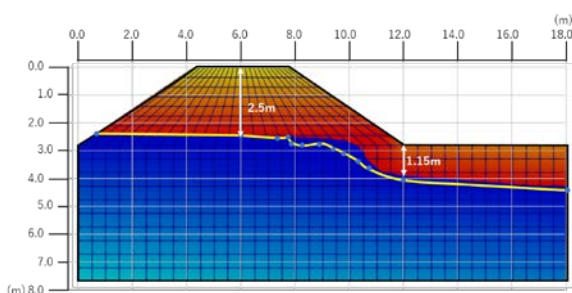
図-5 GPR で得た浸潤線と FEM の結果の比較 Comparison between phreatic line obtained by GPR and FEM result
